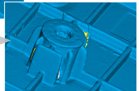
Triangle mesh from a 3D scanner with a resolution of 6 MP (Field of view 480x350 mm)
